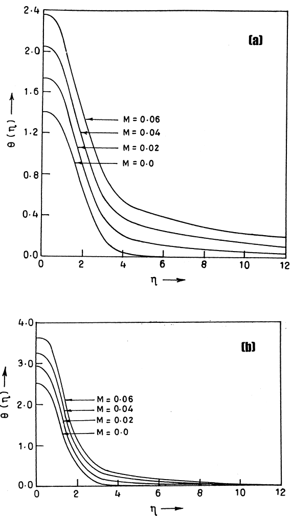
Fig. 3. Temperature profiles: (a) sulphur dioxide ( Pr = 2.0 ); (b) water ( Pr = 7.0 ).
